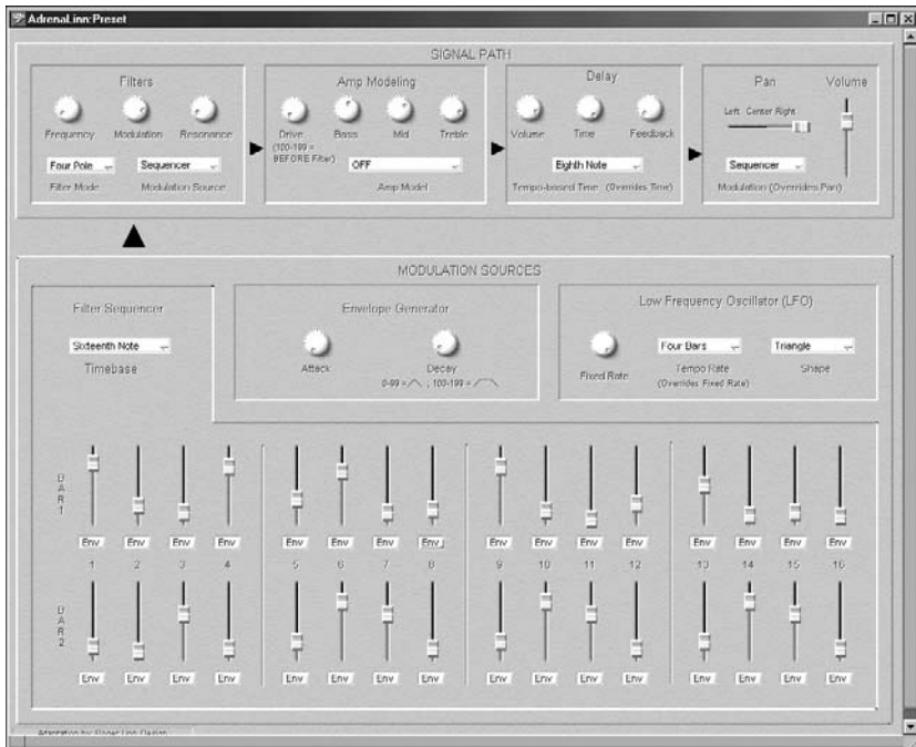
SoundDiver screen for editing AdrenaLinn presets
